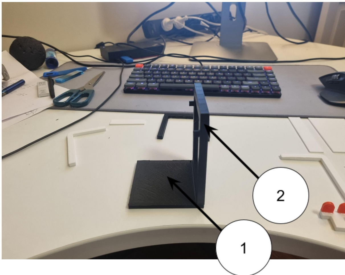
Figure 56: Assembly Step 1
