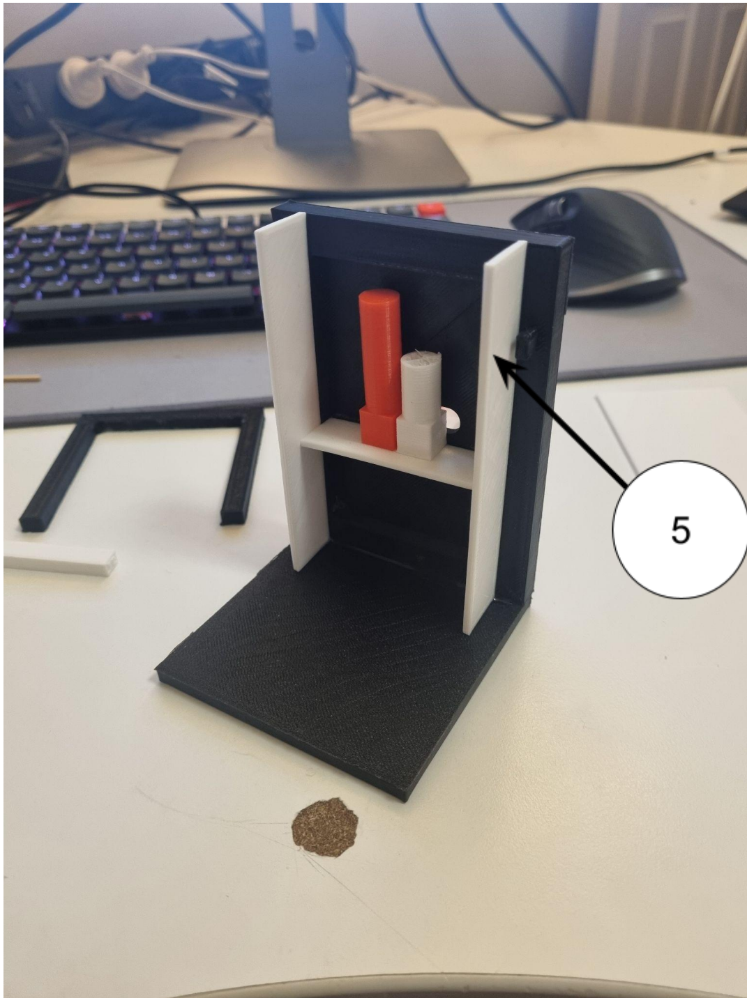
Figure 59: Assembly Step 4
